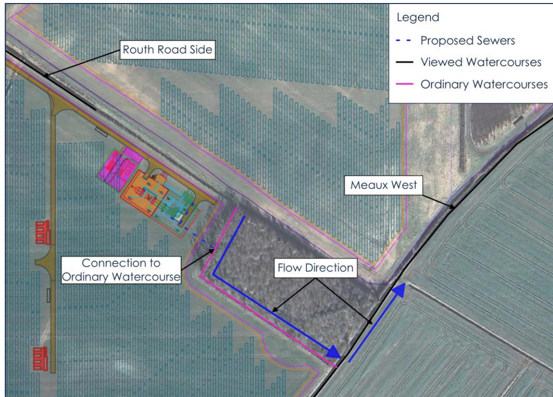
Figure 7-7 Eastern Substation Connection
